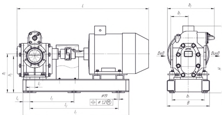
Overall and connecting dimensions of unit pumps AHWM-37,5/2,5, AHWM-30/6, AHWM-22/2,5, AHWM – 19,5/4
