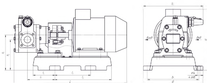
Overall and connecting dimensions of unit pumps AHWM-6,3/25, AHWM-4,0/25, AHWM-2,5/6, AHWM – 1,6/16
